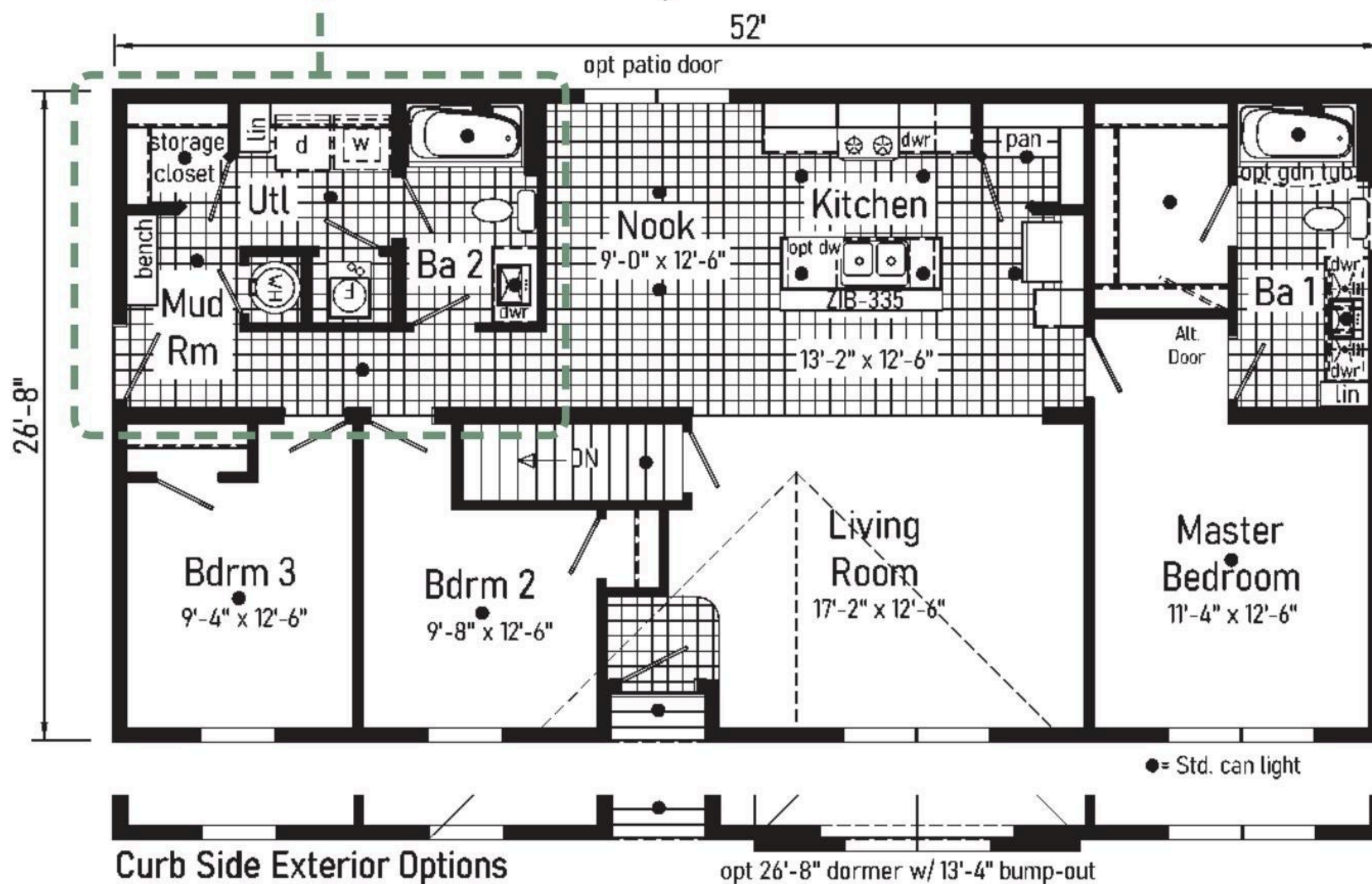
Optional Eat-In Kitchen
