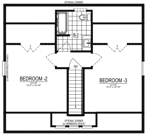
UNFINISHED ATTIC SPACE (Suggested Layout Shown)
