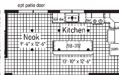
Optional L Kitchen
