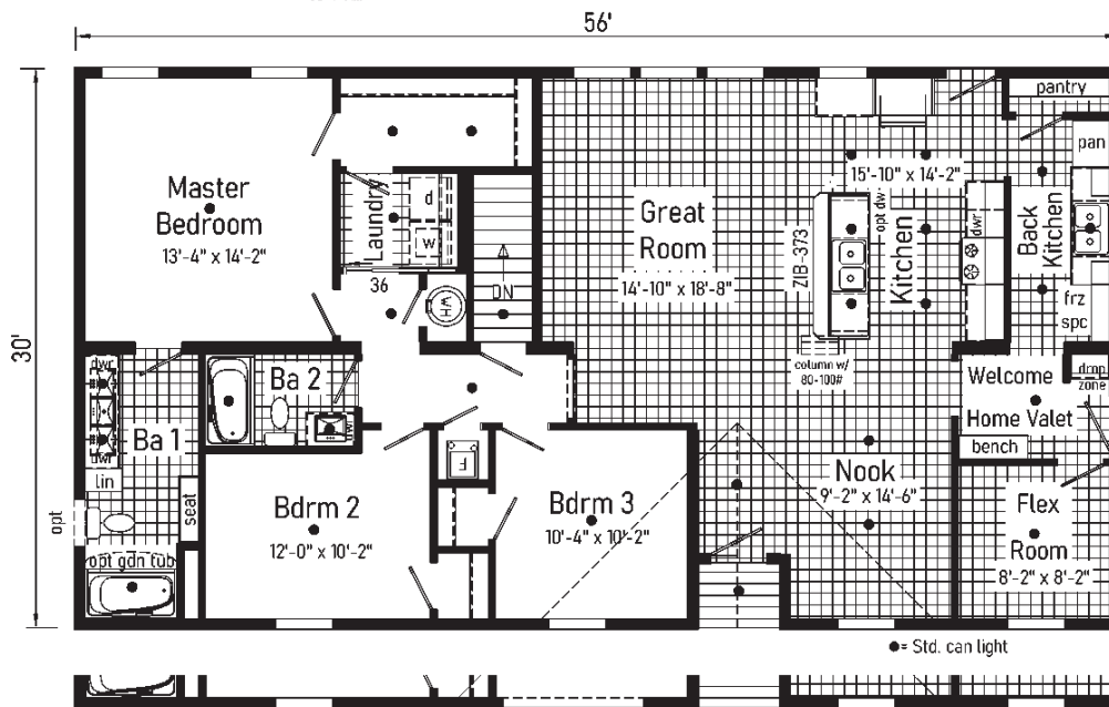
Alternate Chef's Galley
