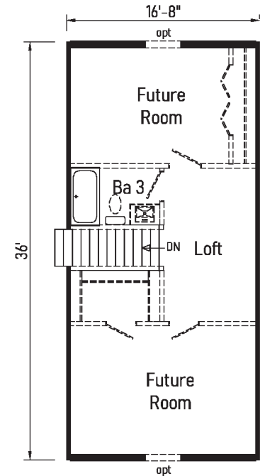
Proposed 2nd Floor for Optional 12/12 Roof
