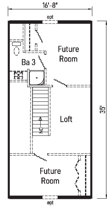
Proposed 2nd Floor for Optional 12/12 Roof
