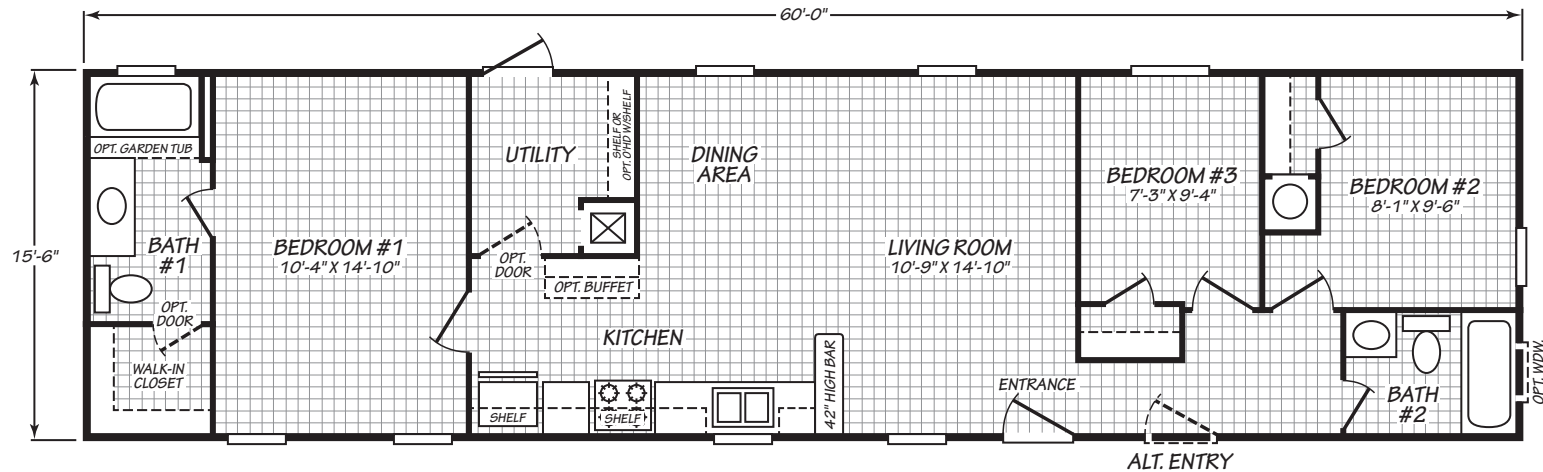
3 BEDROOM PLAN - WITH 4' STRETCH
