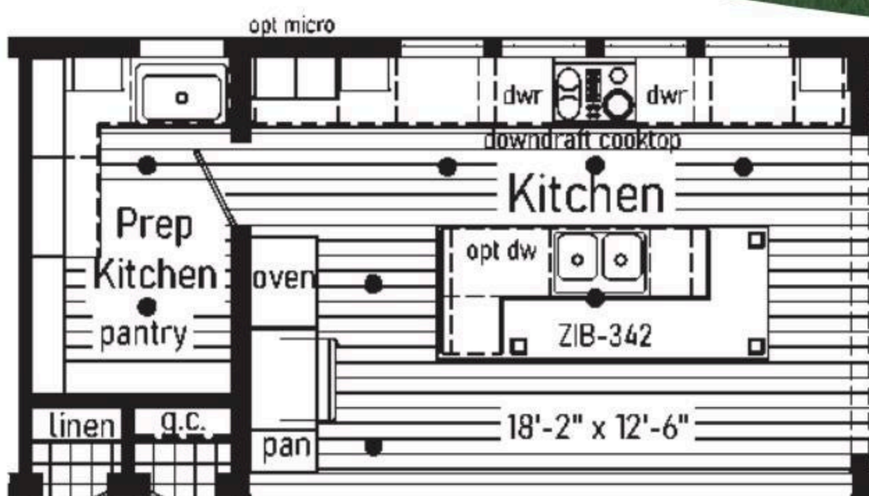
Alternate Kitchen With Optional Down draft Cooktop, Built-In Oven & 4 Window
