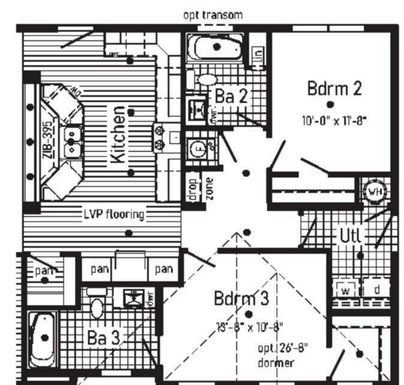
Optional End Utility with 3rd Bath Configuration
