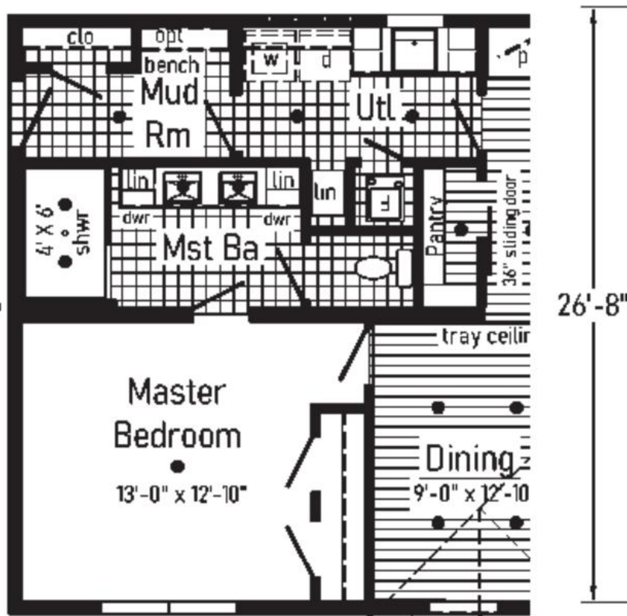
Optional End Entry Utility with 4' x 6' Walk-In Shower
