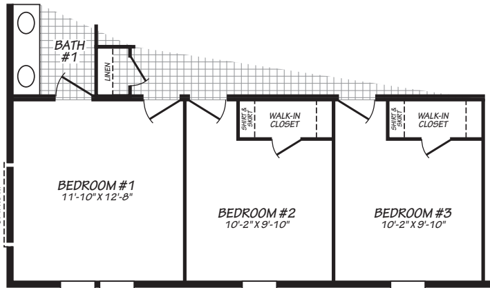
OPTIONAL THREE BEDROOM
